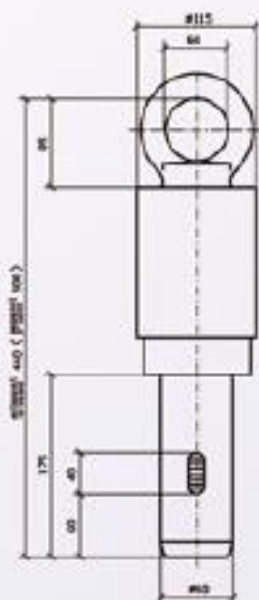
Dimension drawing AL 70/76
