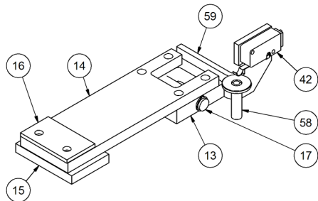
DETAIL SPRING ASS'Y.
