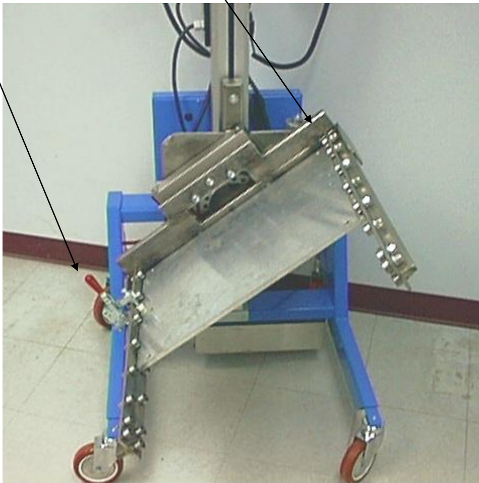
Electric turn device to handle 350 lb dies. Die plate is shown without die.
